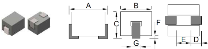
BPH322521W5 Dimensions
